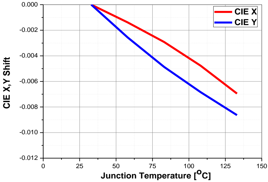
Fig 8. Junction Temp. vs. CIE X, Y Shift, I_F=20\text{mA}
