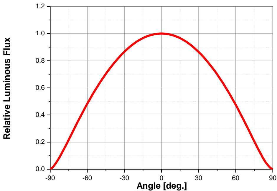
Fig 2. Radiant pattern, T_a=25^\circ\text{C} , I_F=20\text{mA}
