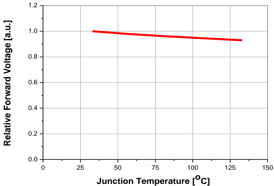
Fig 7. Relative Forward Voltage vs. Junction Temperature, I_F=20\text{mA}
