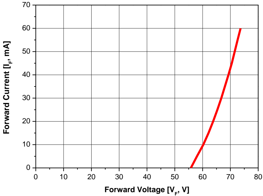
Fig 3. Forward Voltage vs. Forward Current , T_s=25^\circ\text{C}
