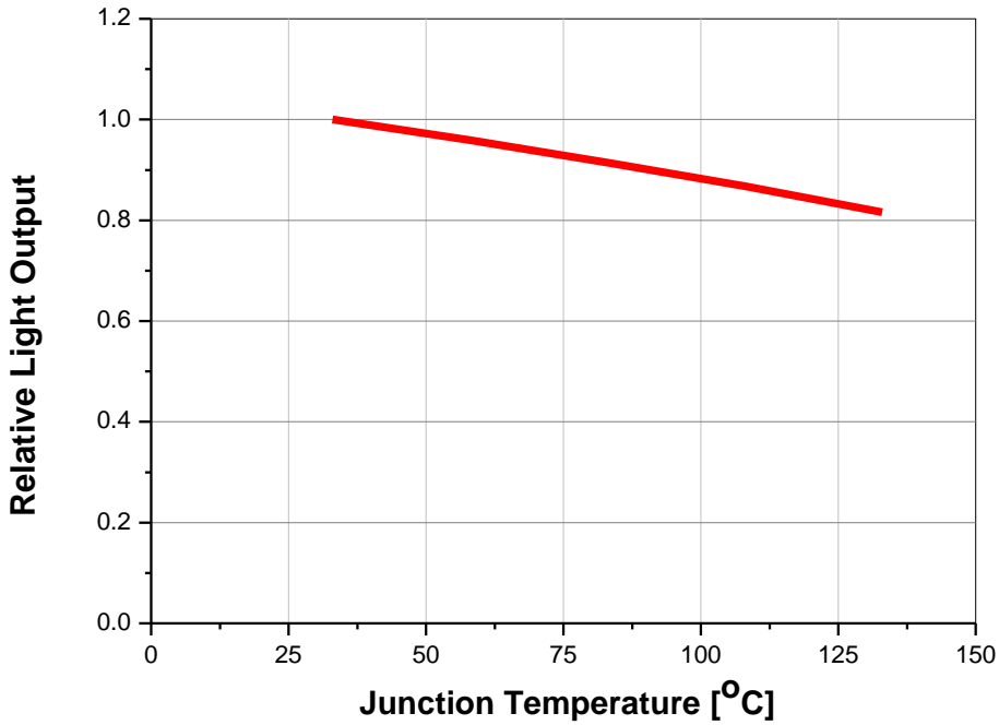
Fig 6. Relative Light Output vs. Junction Temperature, I_F=20\text{mA}
