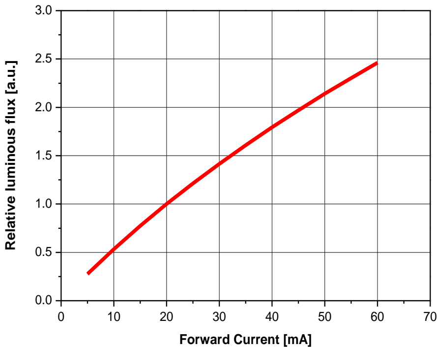
Fig 4. Forward Current vs. Relative Luminous Flux, T_a=25^\circ\text{C}
