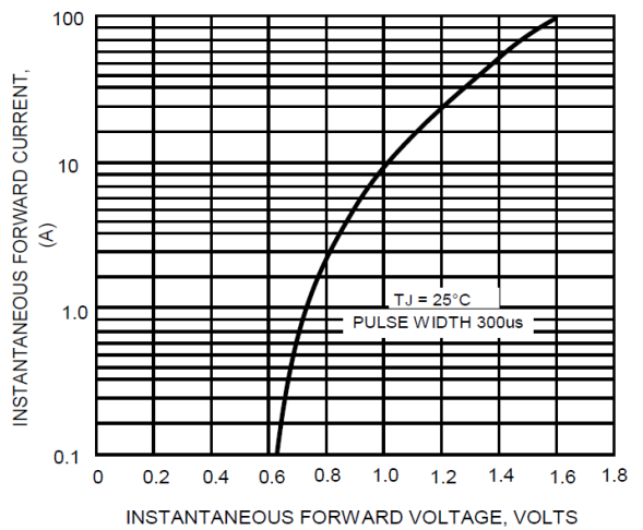
FIG.4-TYPICAL FORWARD CHARACTERISTICS
