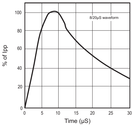
Fig.3 Pulse Waveform
